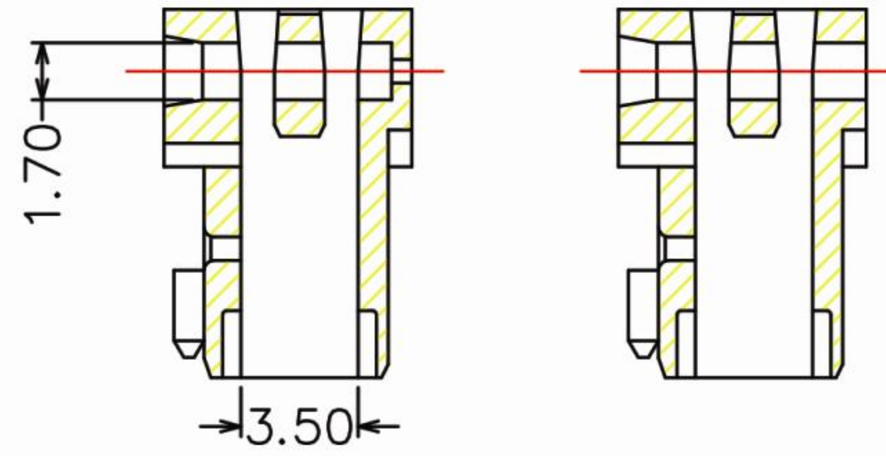
SECTION: B-B
